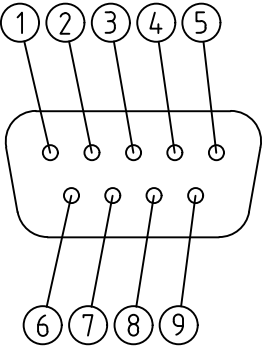
D-sub connector (male)
