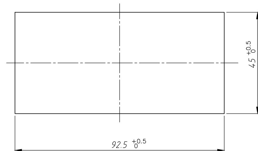
PANEL CUT DIMENSION
